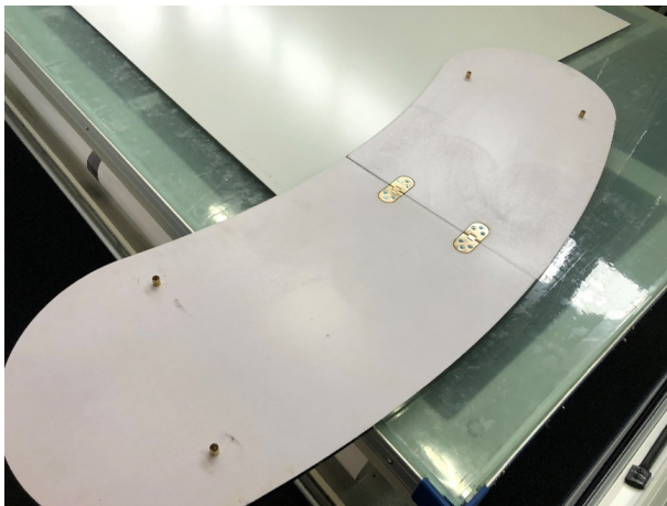
Make sure your top panel is unfolded and the 4 location pins are installed.
